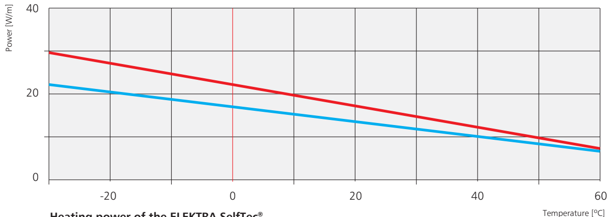
Heating power of the ELEKTRA SelfTec® self-regulating cables in the function of temperature
