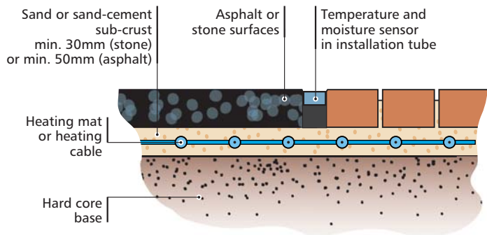
Crosssection of a driveway made of asphalt or paving blocks (installation in a layer of sand bedding)
