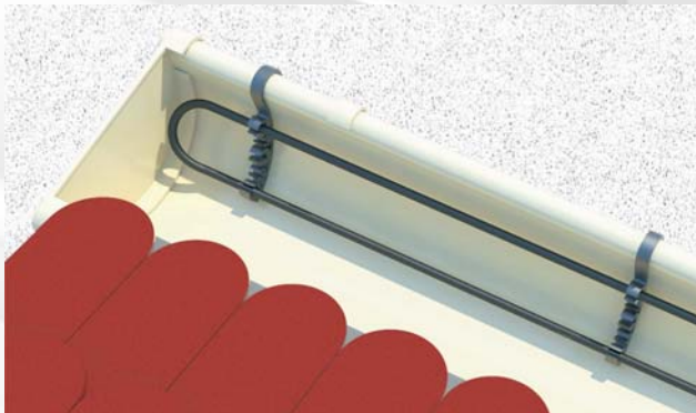
Cable fixing in the gutter
